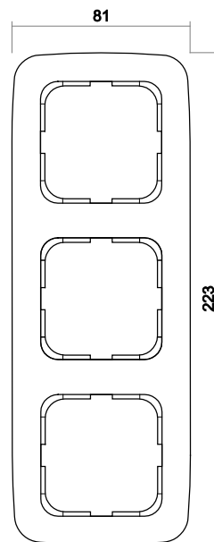
Cover frame 3gang
