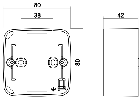
Surface mounted box 1gang
