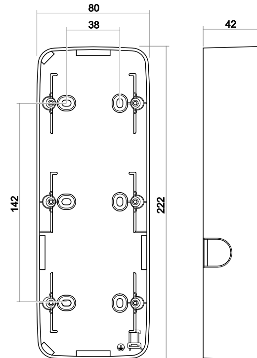
Surface mounted box 3gang
