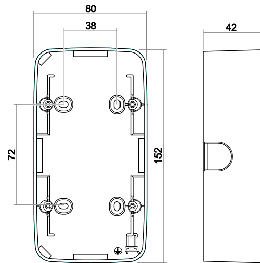
Surface mounted box 2gang
