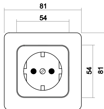
Socket outlet
