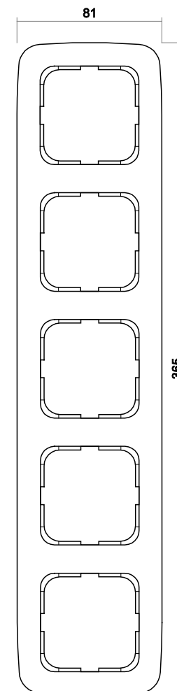
Cover frame 5gang
