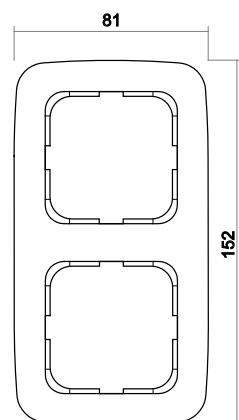
Cover frame 2gang
