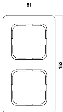
Cover frame 2gang
