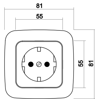
Socket outlet
