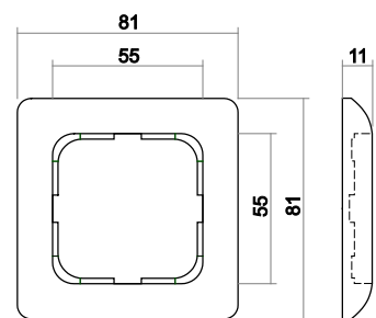
Cover frame 1gang
