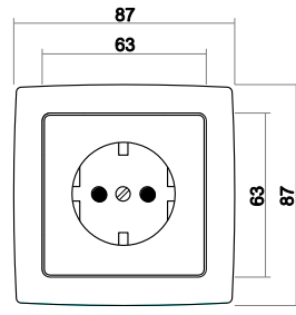
Socket outlet, 1gang
