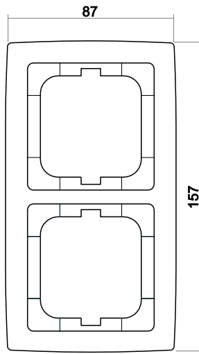
Cover frame, 2gang
