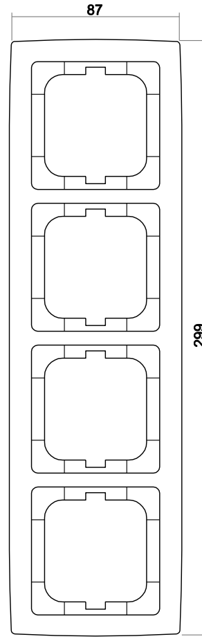
Cover frame, 4gang
