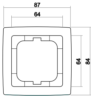
Cover frame, 1gang
