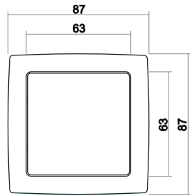
Switch, 1gang
