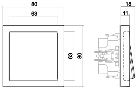
Switch
