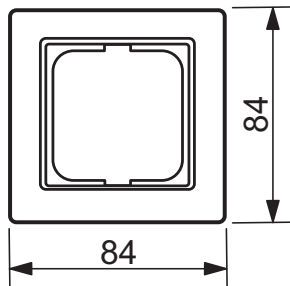
Cover frame, 1gang
