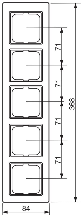
Cover frame, 5gang
