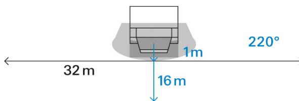
Busch-Watchdog 220 MasterLINE premium
