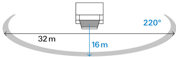
Busch-Watchdog 220 MasterLINE select
