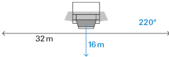
Busch-Watchdog 220 MasterLINE, Busch-Watchdog 220 WaveLINE, Busch-Watchdog 220 MasterLINE KNX, Busch-Watchdog 220 MasterLINE KNX premium
