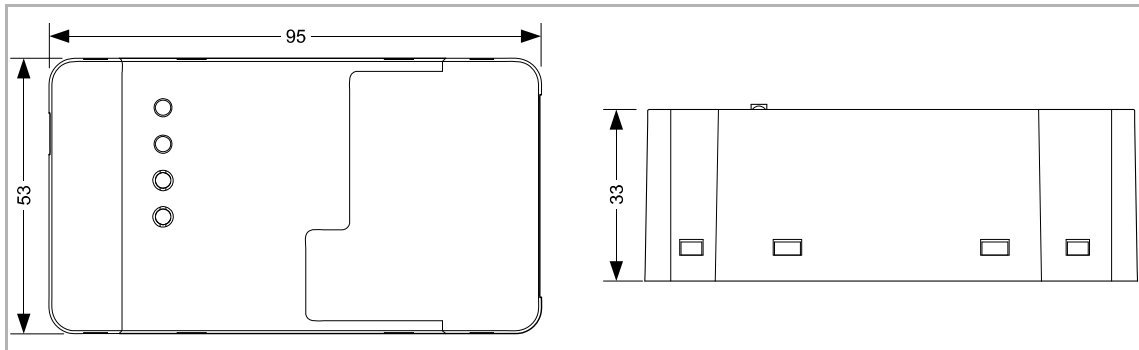
Fig. 3: Dimensions (all dimensions are in mm)
