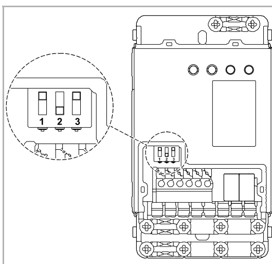
Fig. 7: Dip switch
