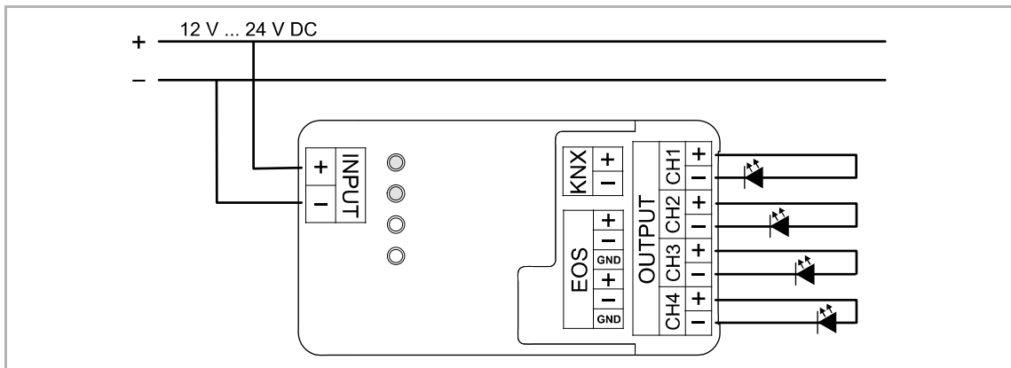
Fig. 4: Electrical connections
