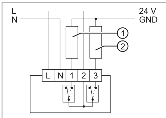
Fig. 7: Control for 24 V
