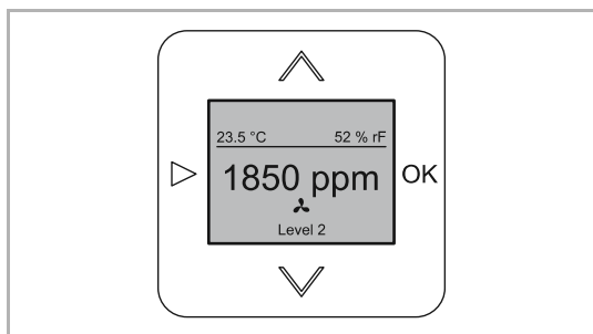
Fig. 20: Fan control: CO 2 threshold value exceeded
